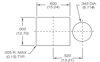
PANEL MOUNTING
