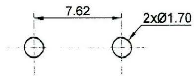
Mounting Detail
