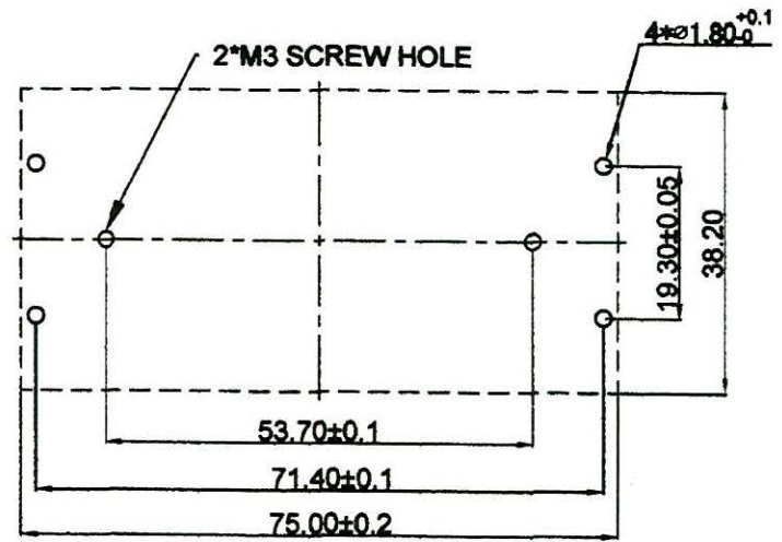
PCB LAYOUT
