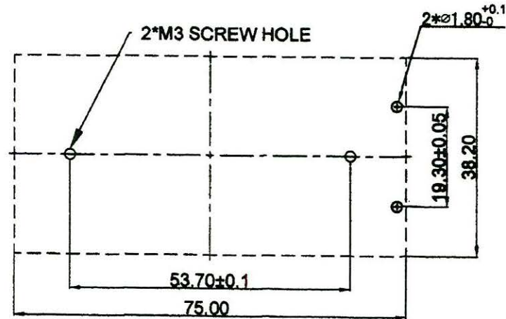
PCB LAYOUT
