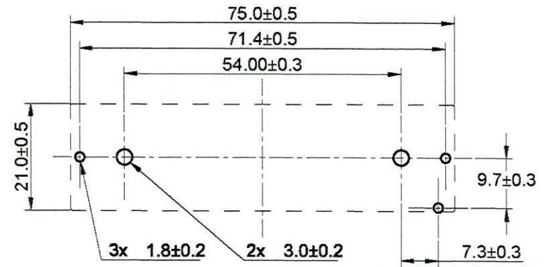
PCB/MOUNTING LAYOUT
