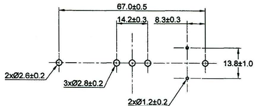
PCB/MOUNTING LAYOUT
