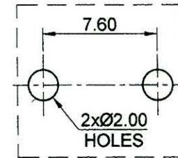
PCB Mounting Layout
