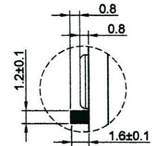
POLARITY PROTECTOR DEVICE DETAIL "A" S=3
