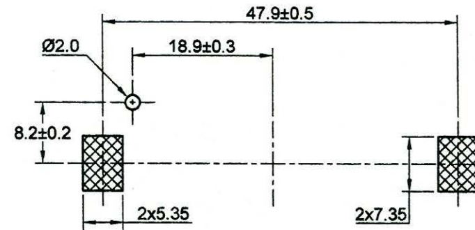
PCB/MOUNTING LAYOUT
