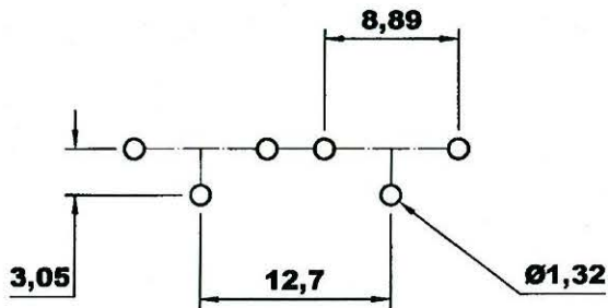
Recommended Layout for 9 Volt Battery Positive and Negative Contact
