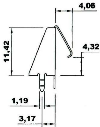
Recommended Layout for 9 Volt Battery Positive and Negative Contact
