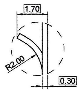
DETAIL "A" S=4
