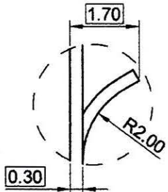
DETAIL "A" S=4
