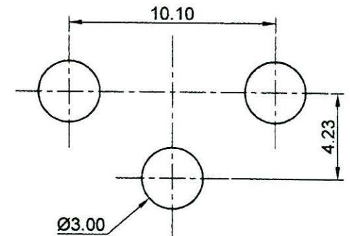
PCB Mounting Layout
