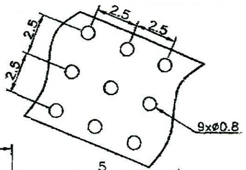
TOP VIEW Bump Detail 5:1
