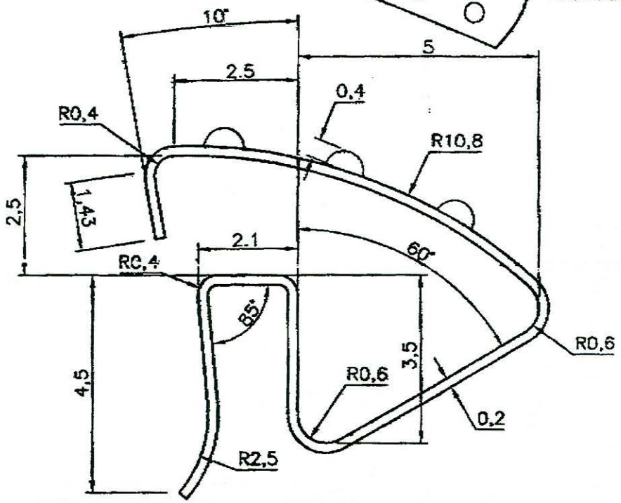
TOP VIEW Bump Detail 5:1
