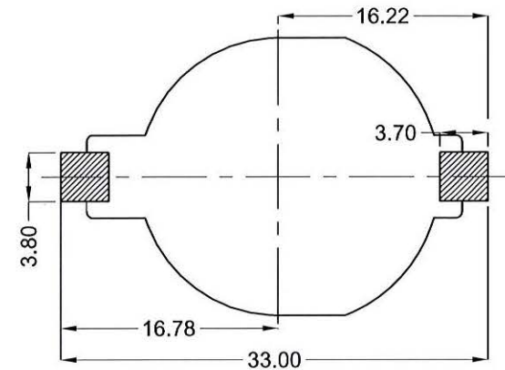
PCB MOUNTING LAYOUT
