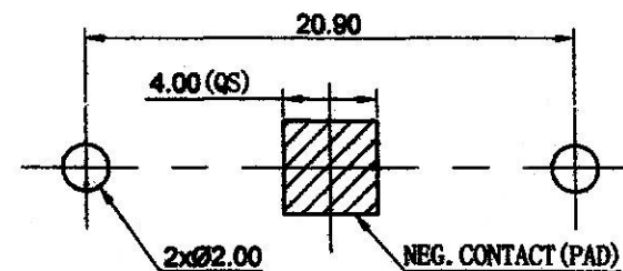
PCB Mounting Layout
