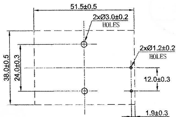
PCB/MOUNTING LAYOUT
