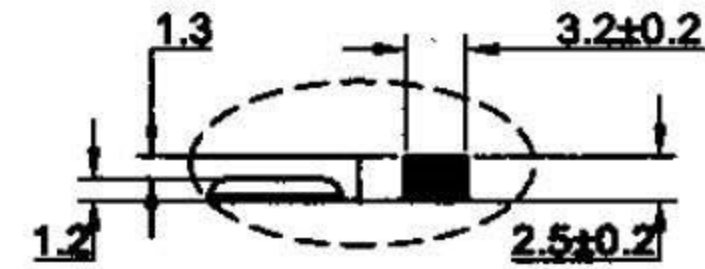
POLARITY PROTECTION DEVICE "A" S=3
