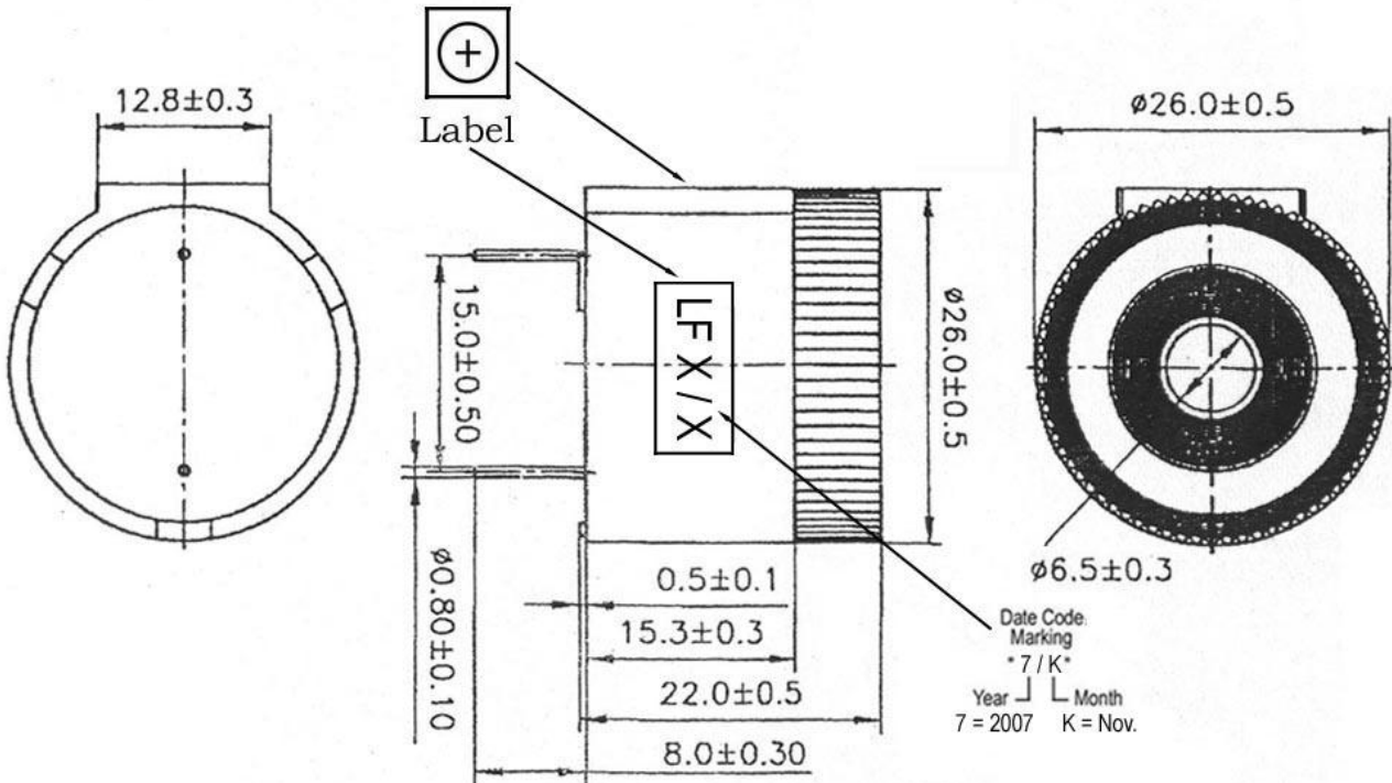
BOTTOM VIEW
