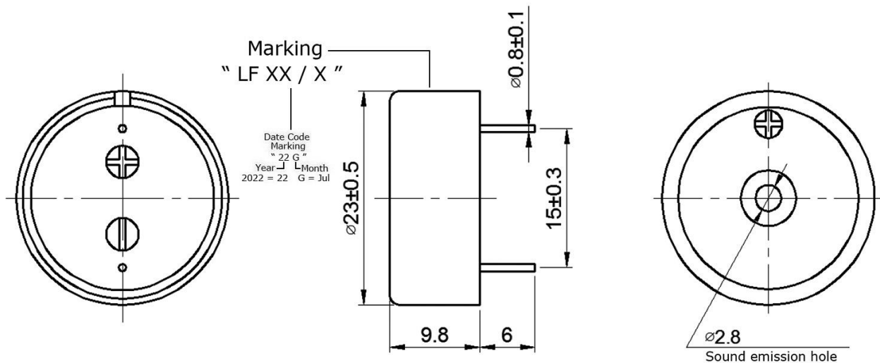
BOTTOM VIEW
