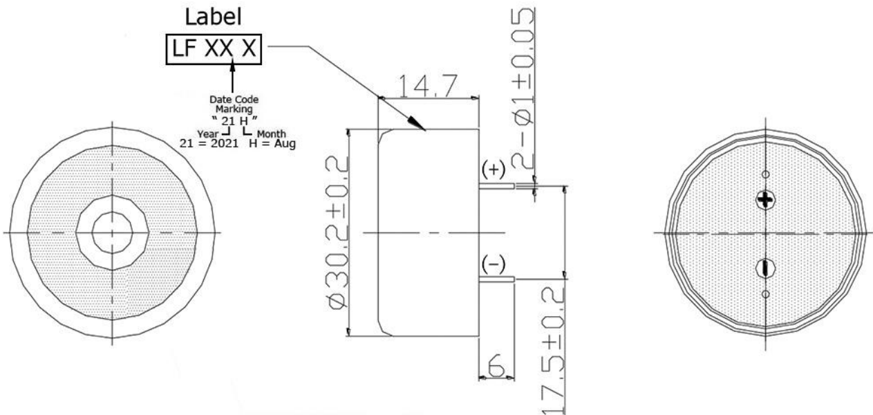
TOP VIEW
