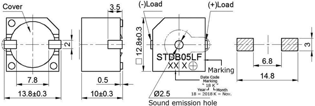
Recommended PCB Land Pattern
