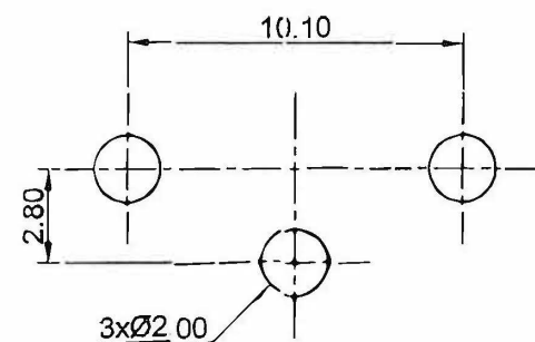
FCB/MOUNTING LAYOUT
