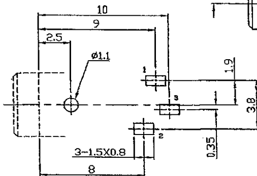
PC BOARD HOLE LAYOUT (BOTTOM VIEW) TOLS : ±0.1
