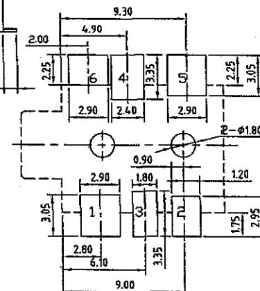
Pin Hole Layout (Jack Bottom View)
