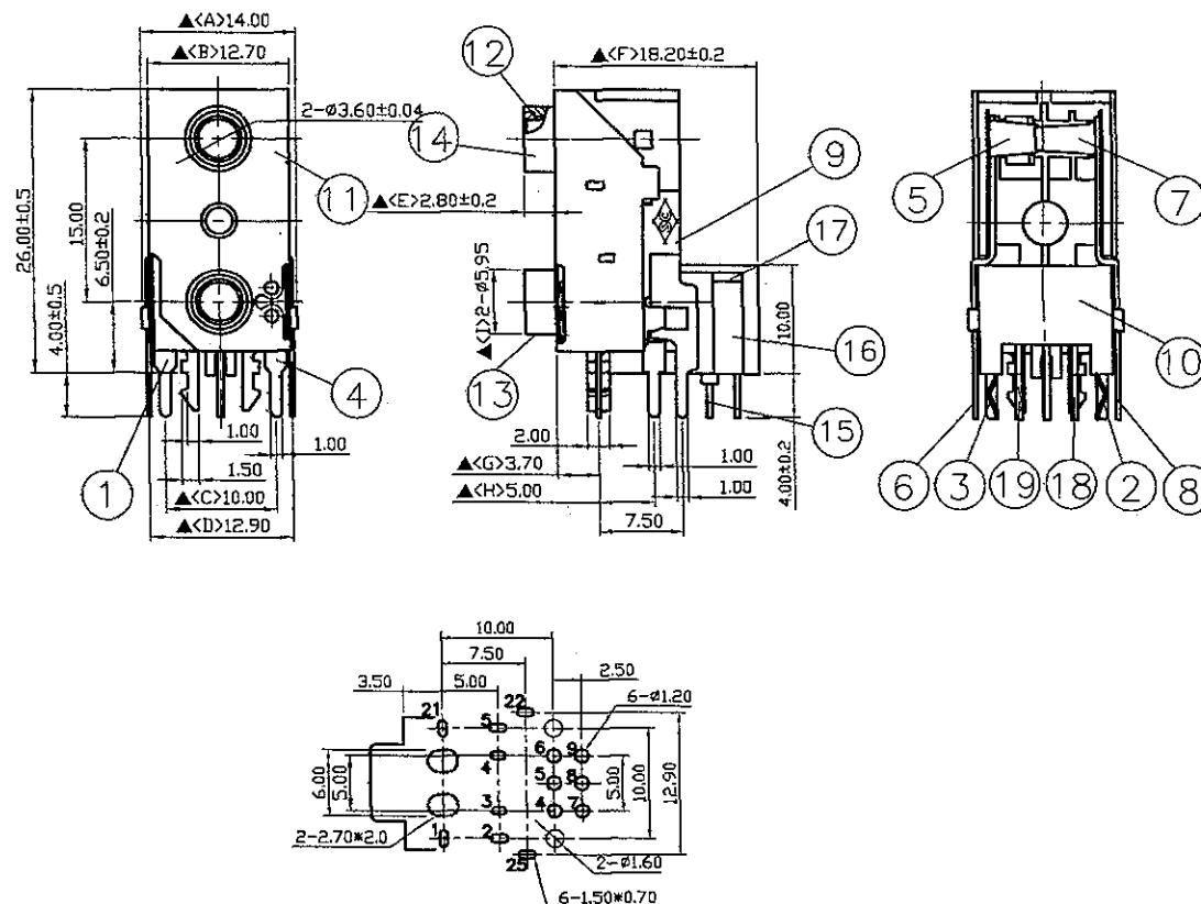
Pin Hole Layout (Jack Bottom View)
