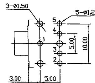
Pin Hole Layout (Jack Bottom View)
