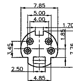
Arrangement of Contact
