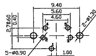
Pin Hole Layout (Jack Bottom View)
