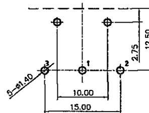
Pin Hole Layout (Jack Bottom View)
