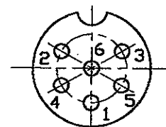
Arrangement of Contact
