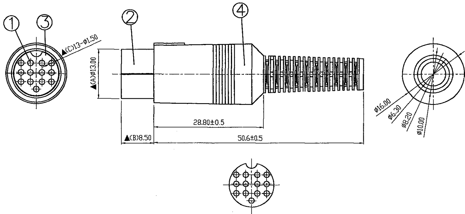
Arrangement of Contact
