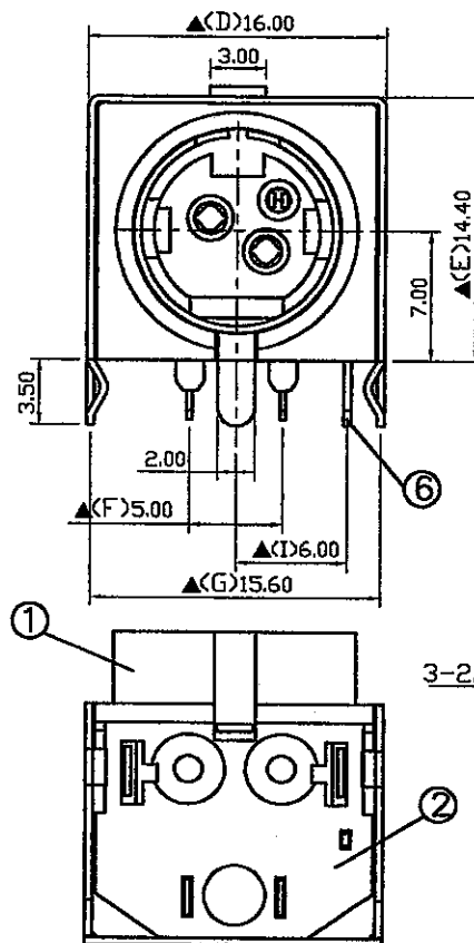
Pin Hole Layout <Jack Bottom View>
