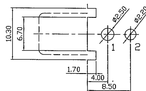
Pin Hole Layout (Jack Bottom View)
