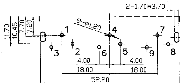
Pin Hole Layout (Jack Bottom View)
