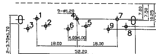
Pin Hole Layout (Jack Bottom View)
