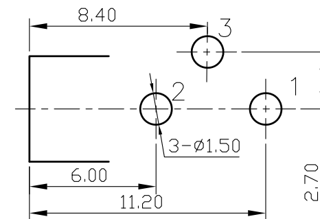
Pin Hole Jack (Jack Bottom View)
