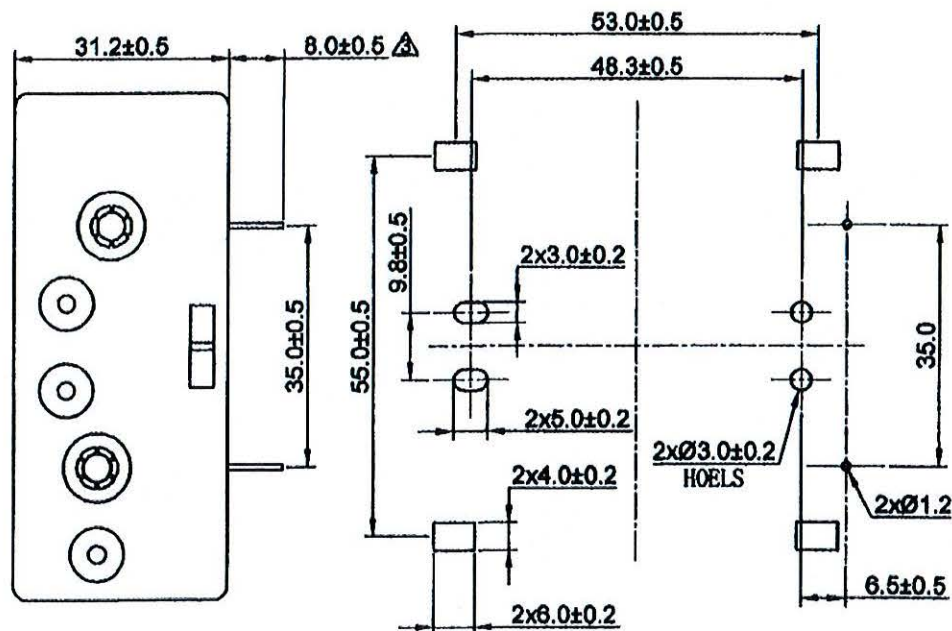
PCB MOUNTING LAYOUT
