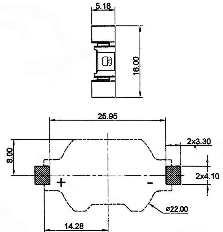
PCB MOUNTING LAYOUT
