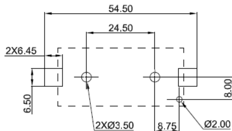
PCB MOUNTING LAYOUT
