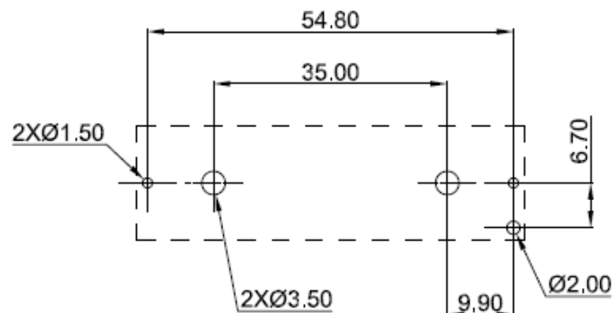
PCB MOUNTING LAYOUT
