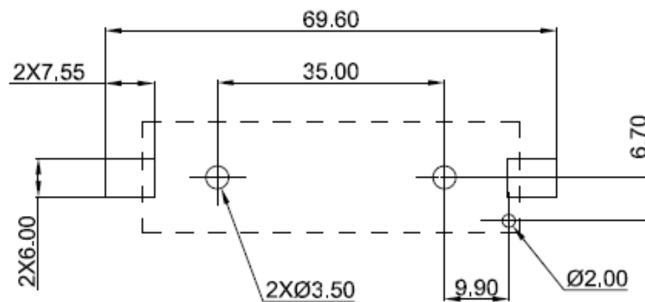
PCB MOUNTING LAYOUT
