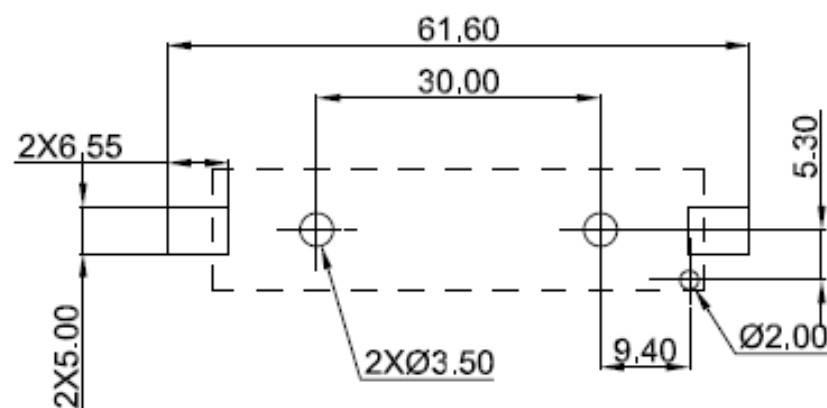
PCB MOUNTING LAYOUT
